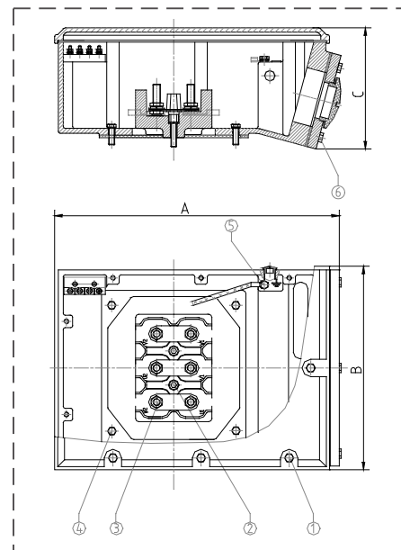
Frame size 315
