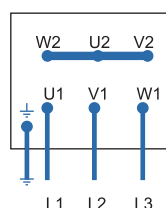
Star connection
