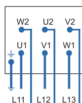
Connection to Star-delta starter
