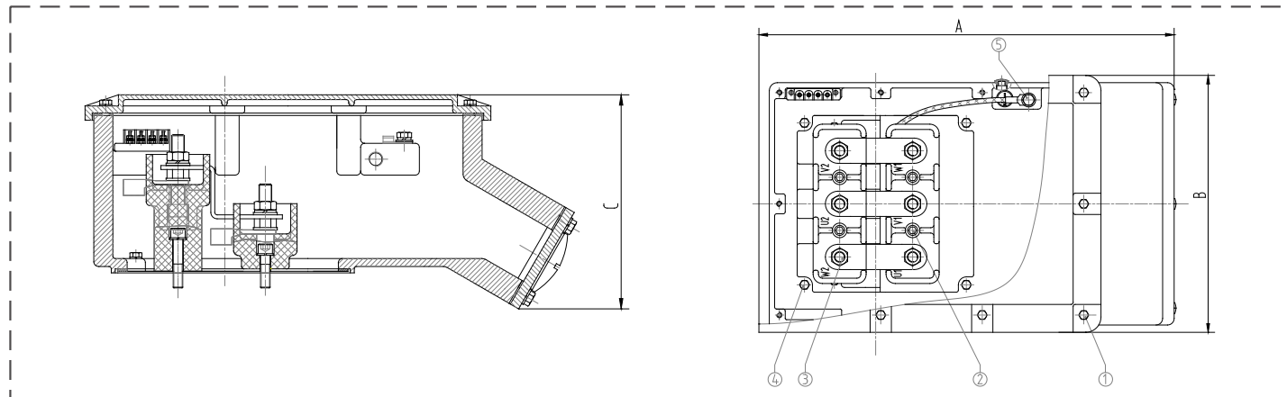
Frame size 355
